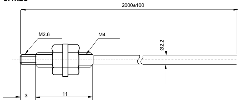
CF/RB3-**
