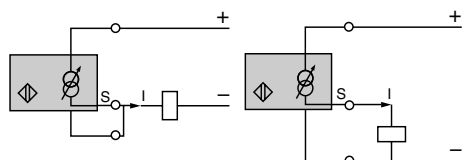
2-wire connection
