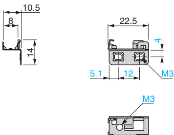
XSZBJ90
