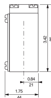
Figure 1 non-plug-in SGA8005 SGO8003 SGC8027 SGI8056 SGO8056 SGI8004 SGO8040 SGO8079
