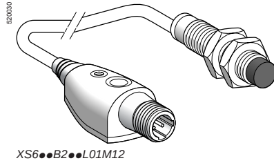
XS6...B2...L01M12
