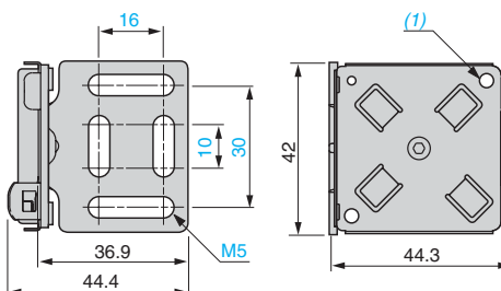
XSZBC90
