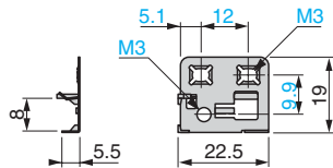
XSZBJ00
