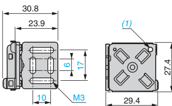
XSZBE90
