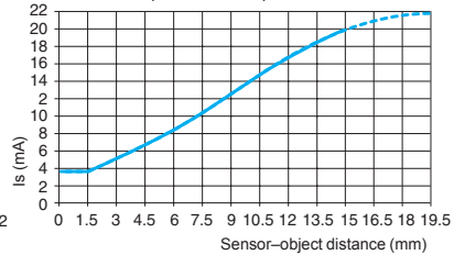
XS4P30AB120
