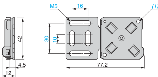
XSZBC00
