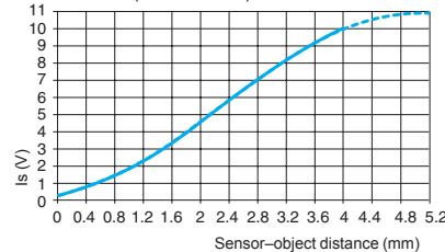
XS4P12AB110
