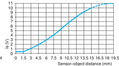
XS4P30AB110
